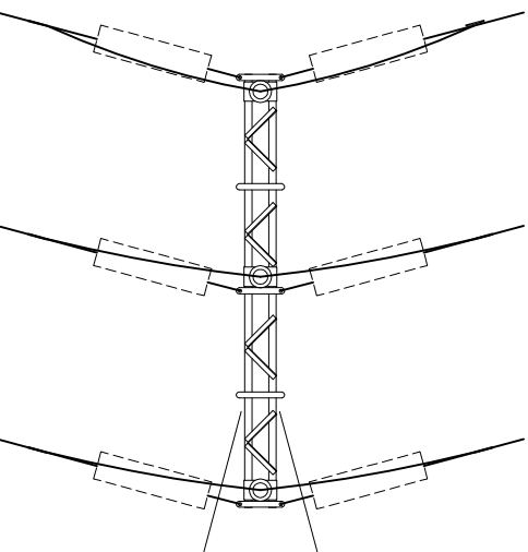
SECTION ANGLE MAX. DEVIATION 30°
