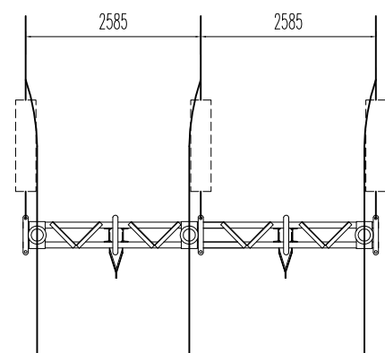
TERMINAL POLE
